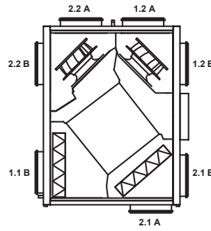
VEX100 - Vertikal LINKS
