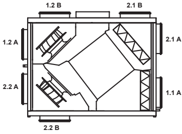
VEX100 - Horizontal/Ceiling LINKS
